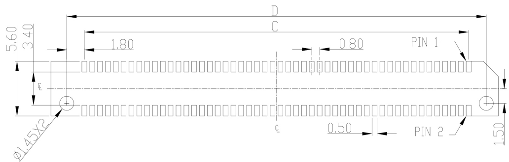
Recommended PC board pattern (TOP VIEW)
